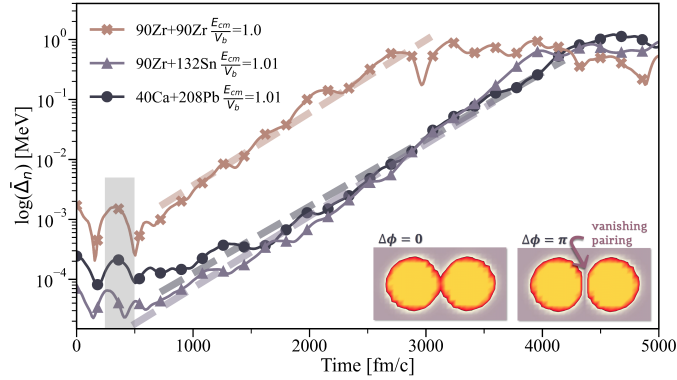
FIG. 1: Modified figure taken from [3]. Figure presents the manifestation of the pairing enhancement after the collision ( t_c \sim gray area). After the contact time the average pairing gap increases exponentially and reaching the value of \sim 1MeV . This phenomenon is generic and is present in different systems. The snapshot presents the vanishing pairing when the two phases of the superfluid state differs by \pi leading to increased barrier for merging and affecting the total kinetic energy of the fragments after separation.
